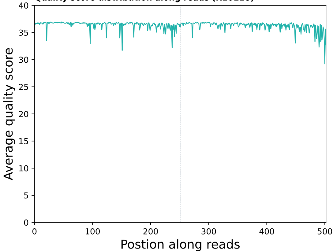
Quality score distribution along reads (R10118)
